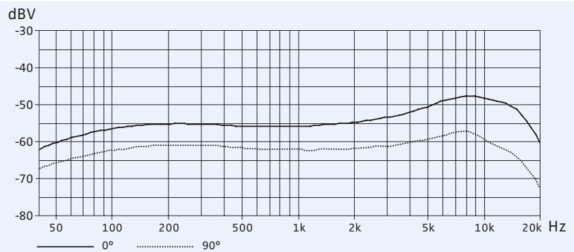
Frequency response curve MME 865-1
