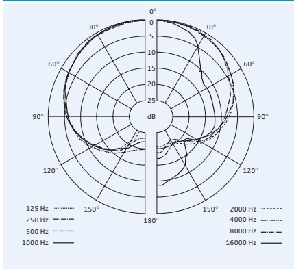
Polar diagram MME 865-1
